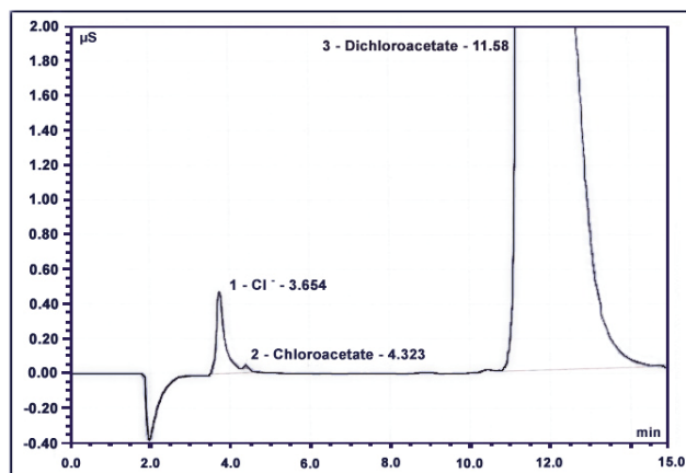
Ion-exchange chromatography chart
