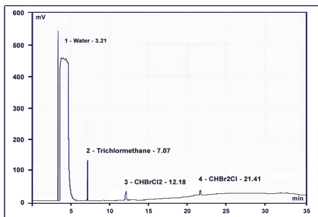
Headspace gas chromatography chart
